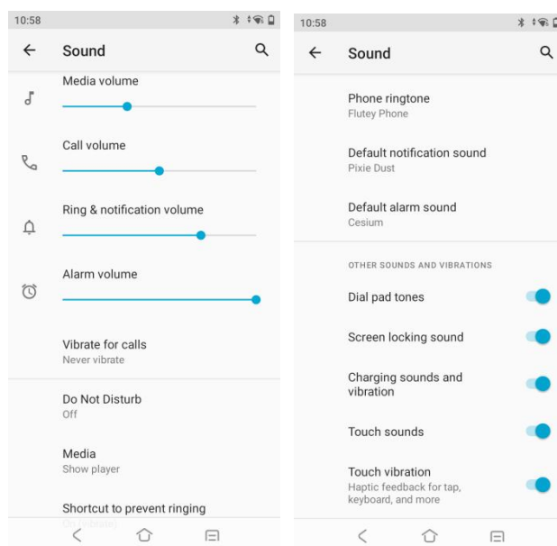
Figure 2- 11 Sound Settings
