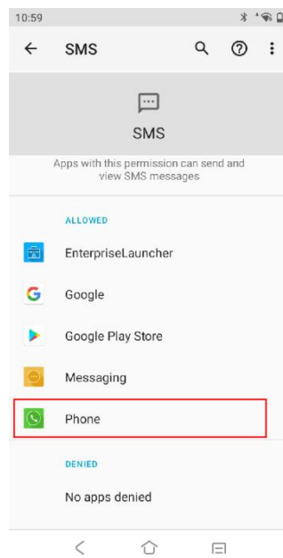
Figure 2- 14 SMS Permissions
