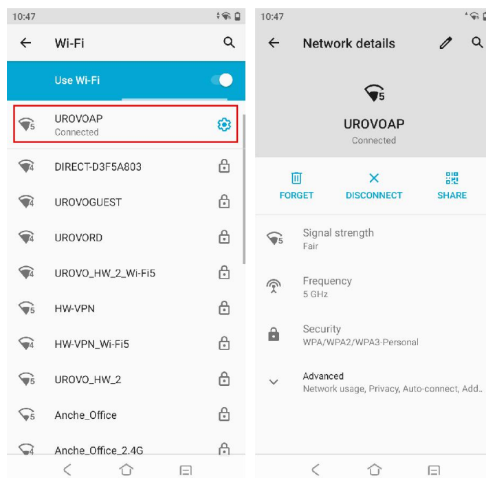
Figure 2- 6 Wi-Fi Connected
