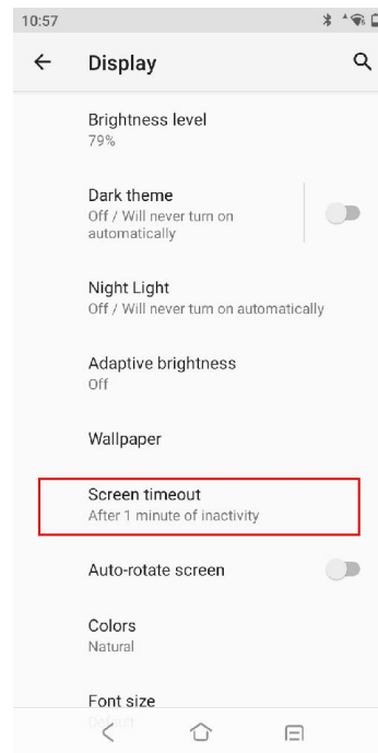
Figure 2- 9 Screen timeout
