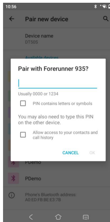
Figure 2- 8 Bluetooth Pairing
