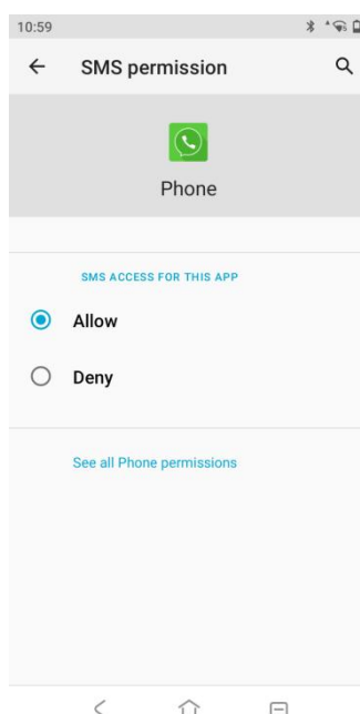
Figure 2- 15 SMS permission
