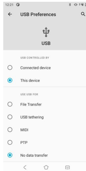
Figure 3- 14 Charging mode
