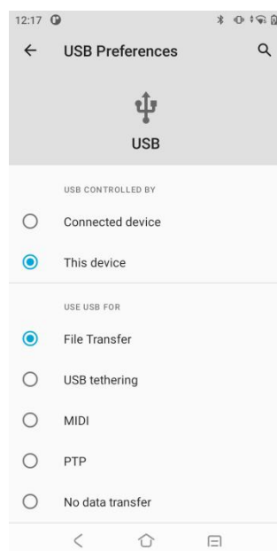
Figure 3- 11 File Transfer
