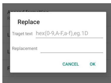
Figure 2- 29 Edit Replace
