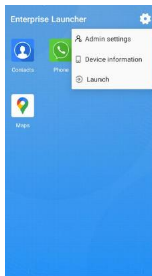
Figure 3- 3 menu
