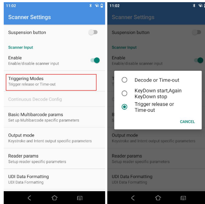
Figure 2- 19 Triggering Mode
