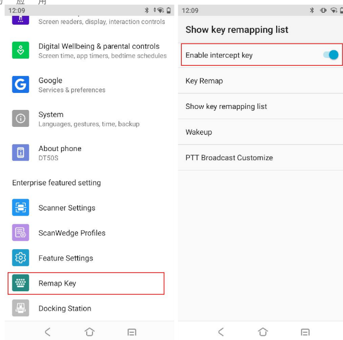
Figure 2- 32 Remap Key
