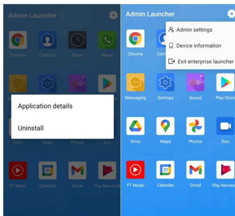
Figure 3- 5 Administrator interface
