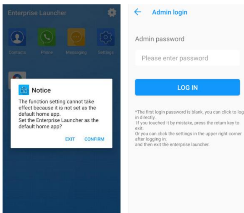
Figure 3- 4 Administration login
