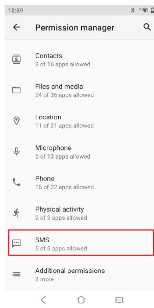
Figure 2- 13 Permission manager
