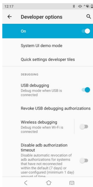
Figure 3- 10 USB debugging
